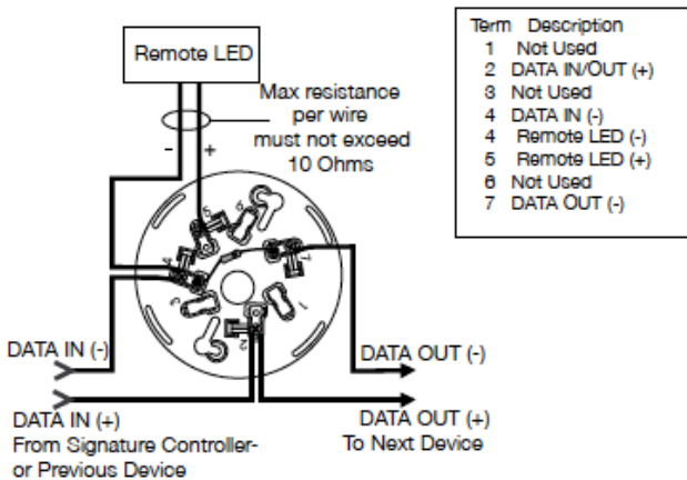
Standard Detector Base, SIGA-SB, SIGA-SB4
